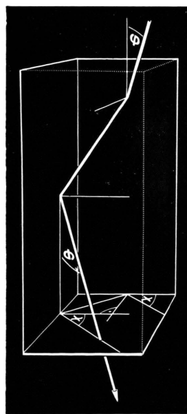
Fig. 2. Schematic drawing of a ray path in a crystalline cone. \varphi is the angle between the incident as well as the emergent ray and the axial direction of the cone. In a tangential plane, here the bottom plate, the projections of the ray and the perpendiculars in the reflection points are drawn. The angle \chi , drawn between the hind edge and the projection of the incident ray is equal to the angle between the projection of the emergent ray and the projection of the second perpendicular of incidence.
